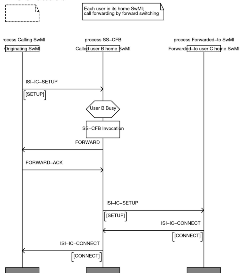
Figure A.1: Call forwarding busy by forward switching
